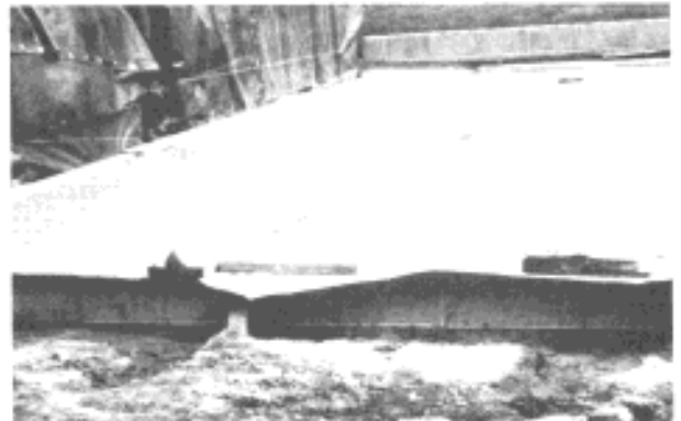
Slab-on-grade covered with waterproof paper for curing.
